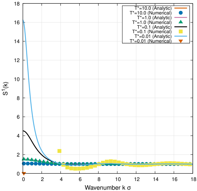
Decoupled Mode S^1(k)
