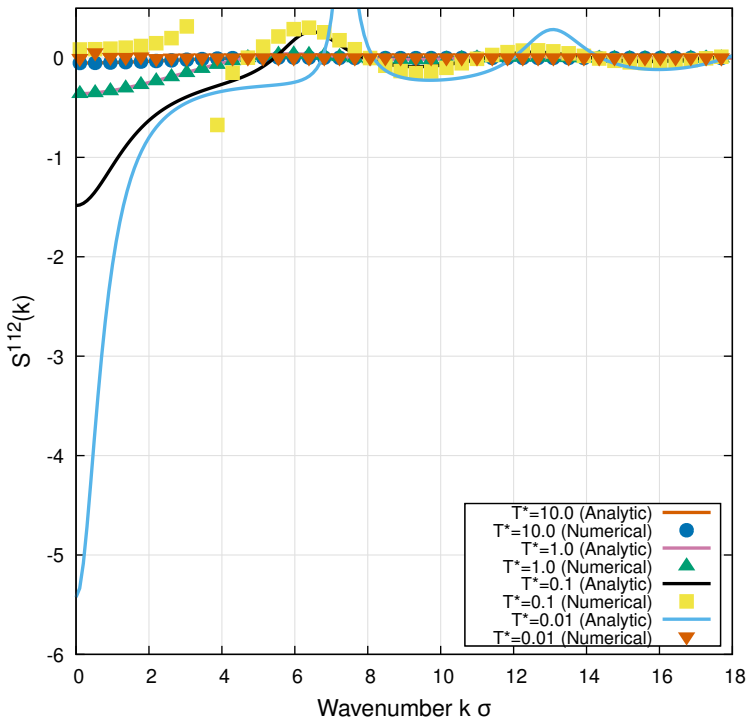
Dipolar Anisotropy S^{112}(k)
