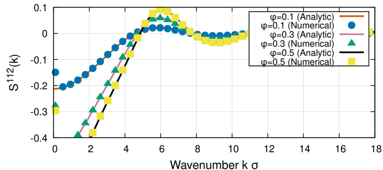
S^{112}(k) at T^* = 1.0
