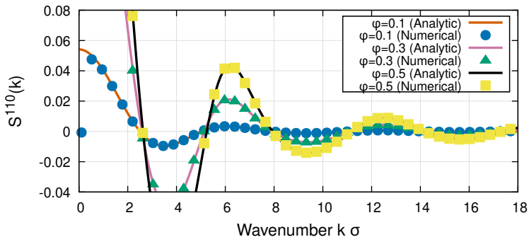
S^{110}(k) at T^* = 1.0
