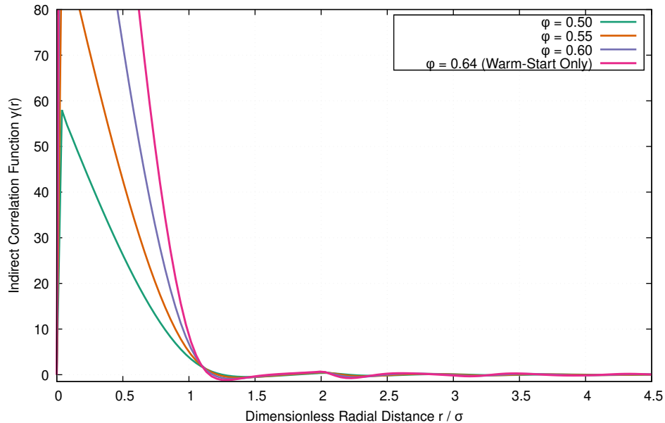
Indirect Correlation Function \gamma(r) Profiles (Percus-Yevick Hard Spheres, N_{\text{nodes}}=4096 )
