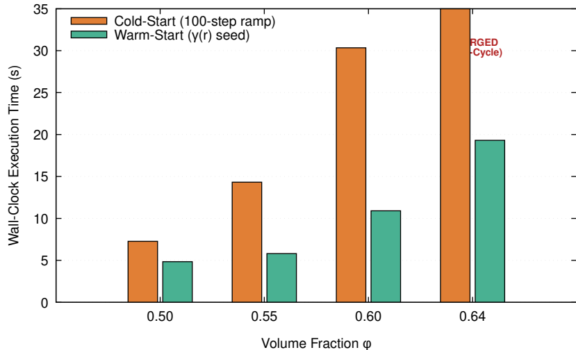
Execution Time Comparison: Cold-Start vs Warm-Start (Percus-Yevick Hard Spheres, N_{\text{nodes}}=4096 )
