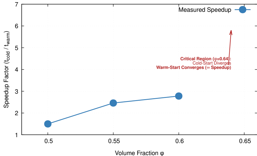
Warm-Start Speedup Factor vs. Volume Fraction \phi (Percus-Yevick Hard Spheres, N_{\text{nodes}}=4096 )
