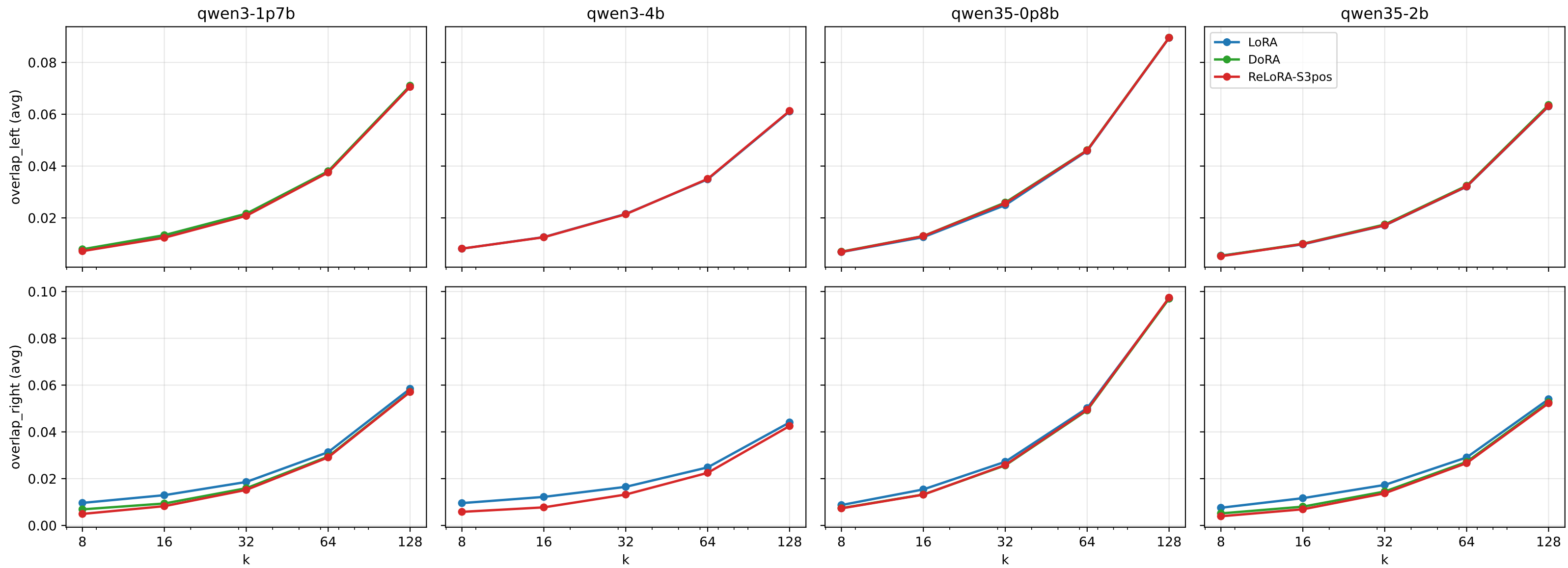
Fig_B — Subspace overlap of top-k(W0) and top-k( \Delta W ) ( \|U1^T U2\|_F^2 / k )
