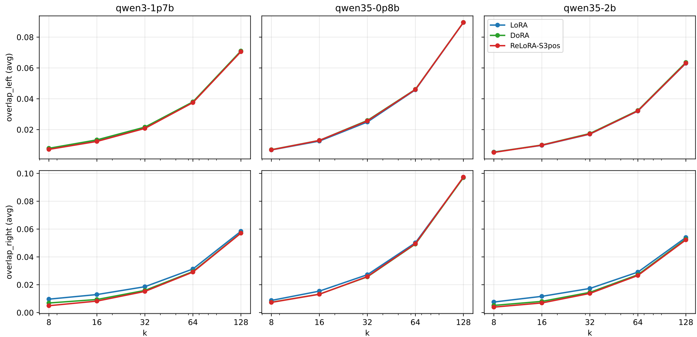
Fig_B — Subspace overlap of top-k(W0) and top-k( \Delta W ) ( \|U_1^T U_2\|_F^2 / k )
