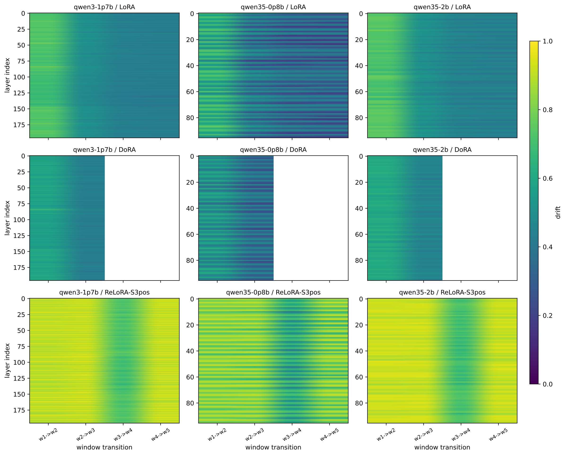
Fig_C — Per-window subspace drift (1 - overlap_left at k=32)
