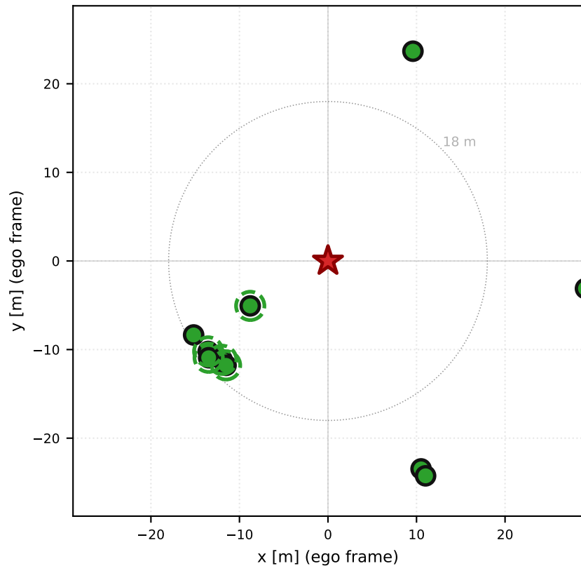
Decoupled typed-budget (Ours, 12 dyn + 4 rel) 6 / 6 near agents selected · pred err = 0.20 m
