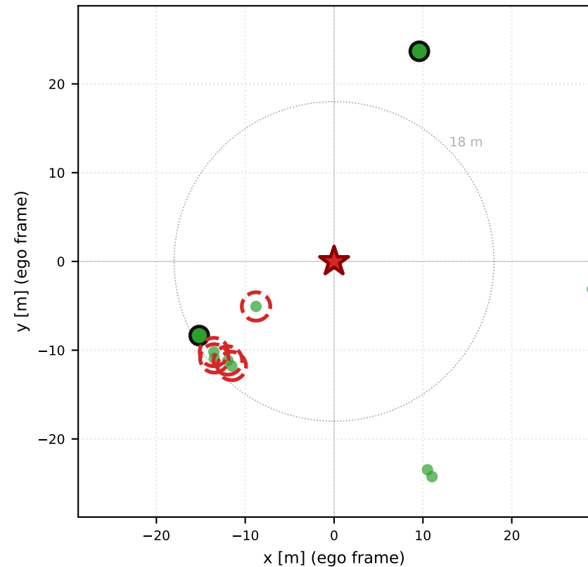
Object+Relation-16 (naive, shared top-k) 1 / 6 near agents selected · pred err = 3.46 m
