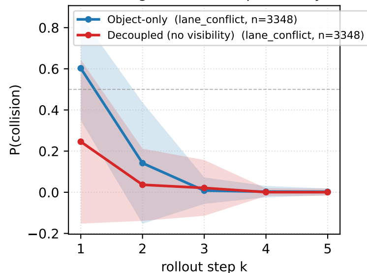
(A) Imagined collision probability
