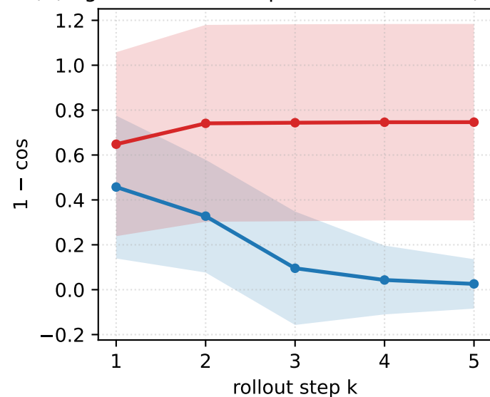
(C) Ego-slot cosine step distance 1 - \cos(e_t, e_{t+1})
