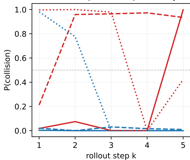
(E) Per-step collision probability
