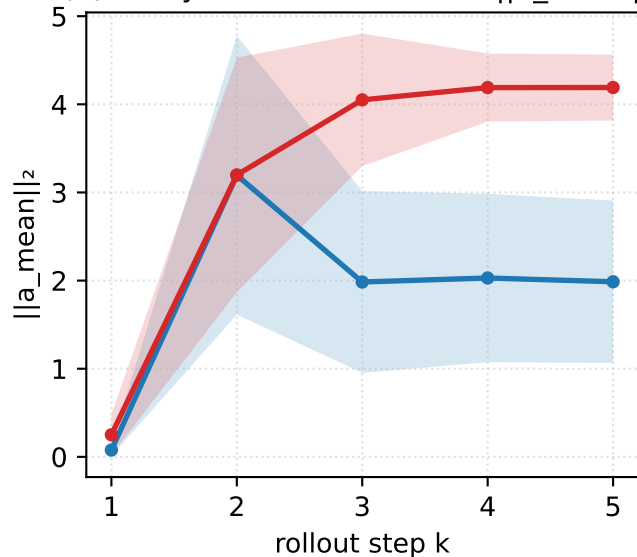
(B) Policy mean action norm \|a_{\text{mean}}\|_2
