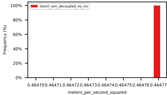
abs_ego_lon_acceleration_within_bounds
