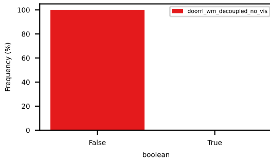
speed_limit_compliance
