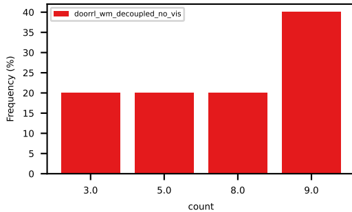
avg_ego_lane_change_duration
