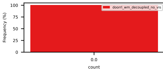
number_of_at_fault_collisions_with_objects
