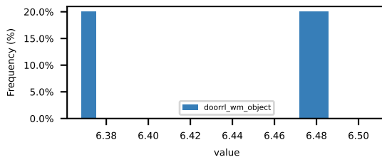
mean_collision_energy_with_objects
