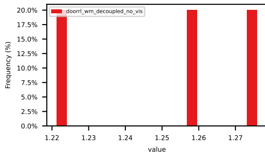
min_violation_of_speed_limit_compliance
