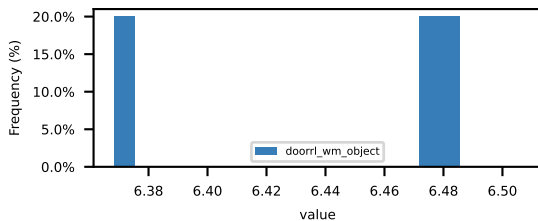
min_collision_energy_with_objects
