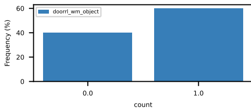
min_collision_energy_with_objects
