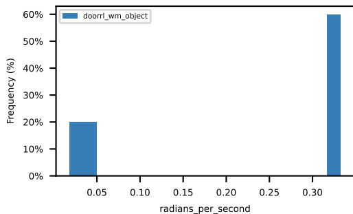
avg_ego_yaw_rate
