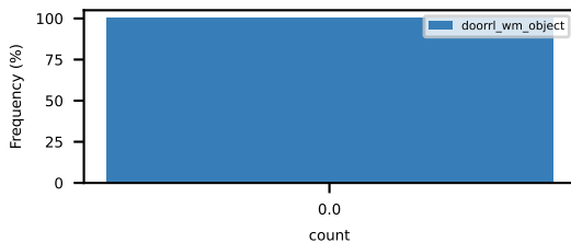
number_of_at_fault_collisions_with_objects
