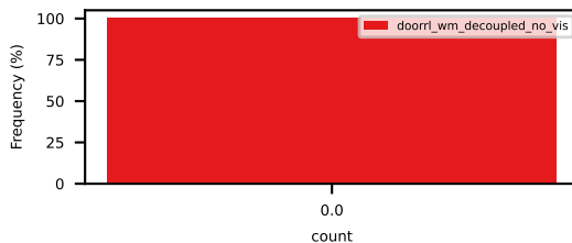
max_collision_energy_with_objects
