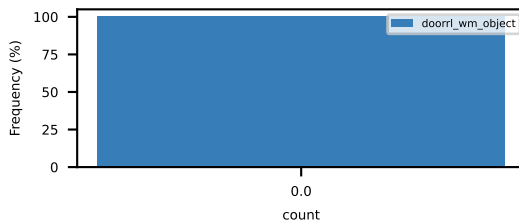
max_collision_energy_with_objects
