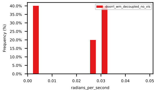
p90_ego_yaw_rate
