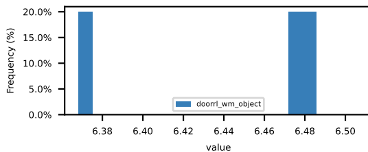
mean_collision_energy_with_objects
