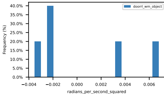
abs_ego_yaw_acceleration_within_bounds
