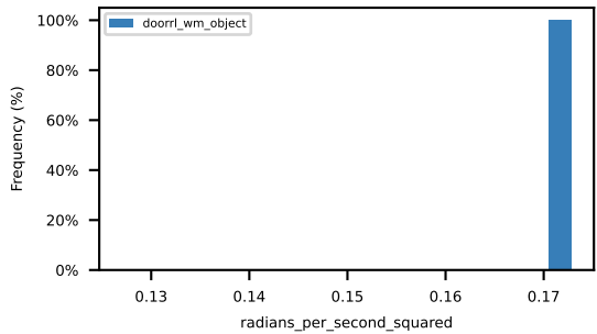
p90_ego_yaw_acceleration
