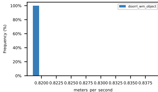
mean_violation_of_speed_limit_compliance
