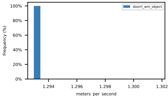
speed_limit_compliance
