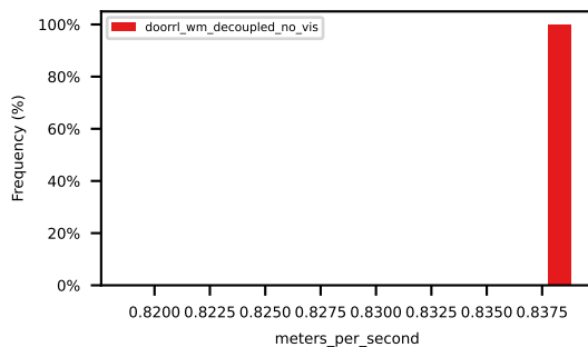
mean_violation_of_speed_limit_compliance
