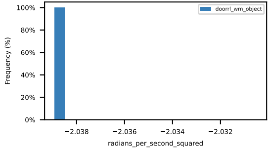
min_ego_yaw_acceleration
