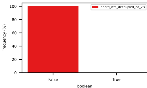
speed_limit_compliance
