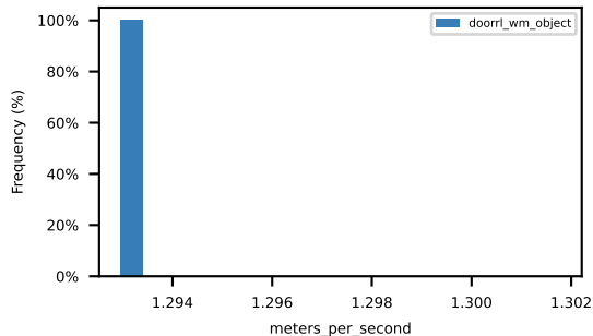
mean_violation_of_speed_limit_compliance
