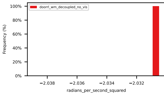
min_ego_yaw_acceleration
