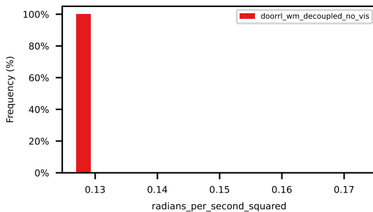
p90_ego_yaw_acceleration
