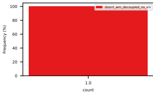
min_violation_of_speed_limit_compliance
