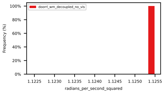
max_ego_yaw_acceleration
