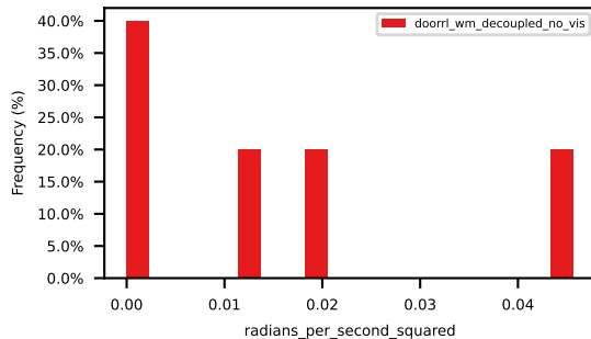
p90_ego_yaw_acceleration
