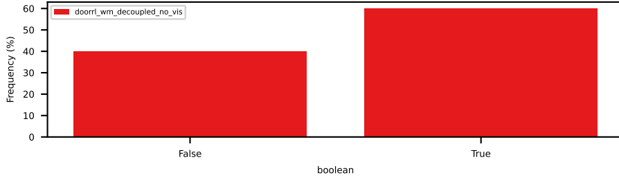
number_of_at_fault_collisions_with_VRUs
