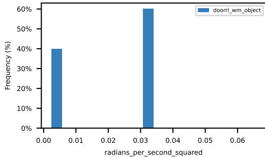
avg_ego_yaw_acceleration
