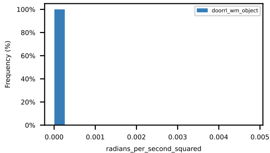
abs_ego_yaw_acceleration_within_bounds
