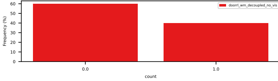
min_collision_energy_with_vehicles
