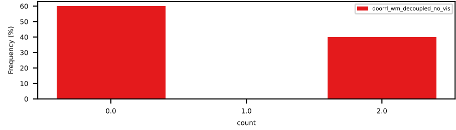
number_of_at_fault_collisions_with_vehicles
