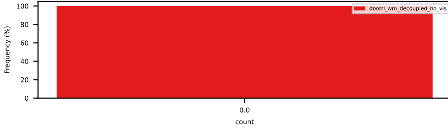
number_of_at_fault_collisions_with_objects
