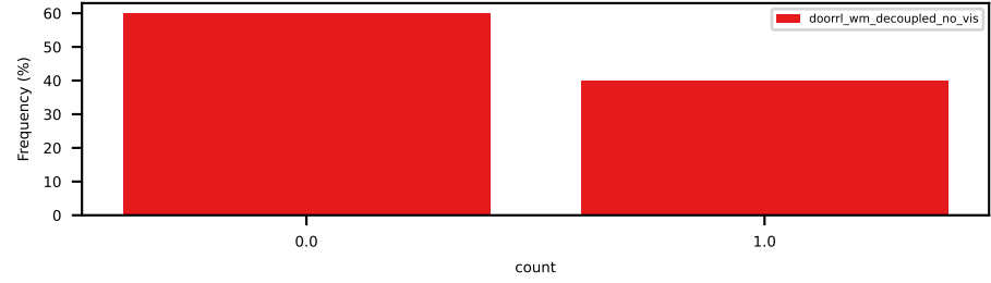
max_collision_energy_with_vehicles
