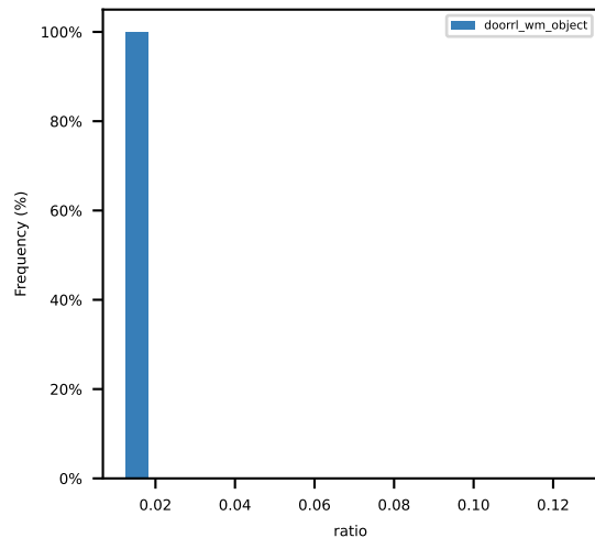
ego_expert_progress_along_route_ratio
