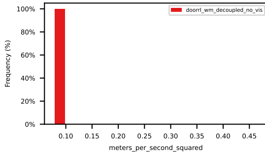
abs_ego_lon_acceleration_within_bounds
