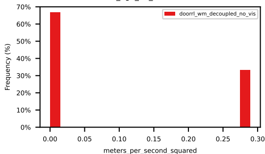
avg_ego_lat_acceleration
