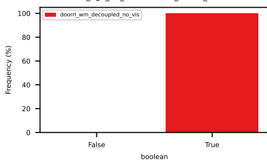
abs_ego_lat_acceleration_within_bounds
