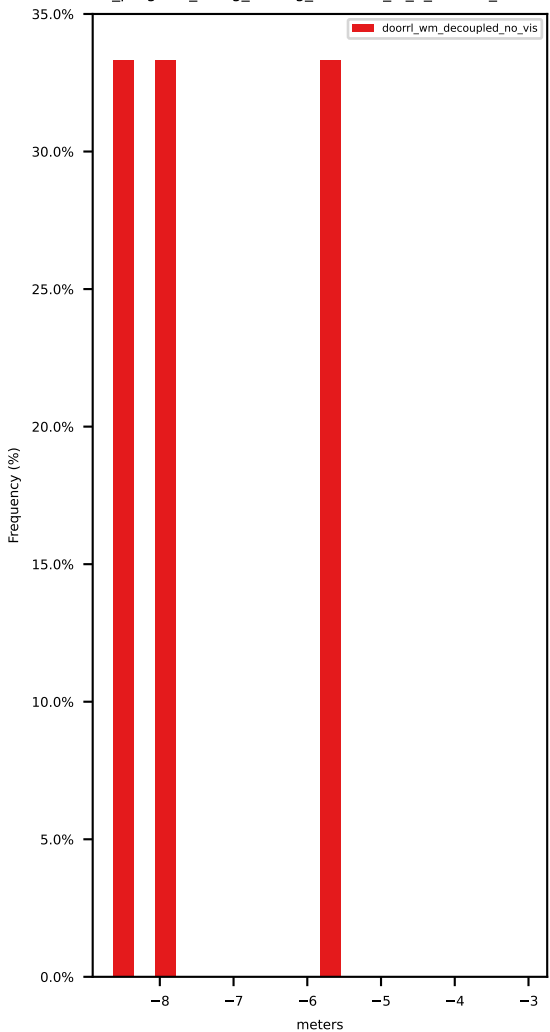
min_progress_along_driving_direction_in_1_second_interval
