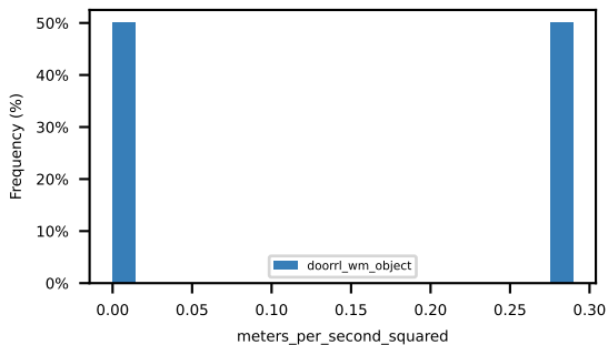
avg_ego_lat_acceleration
