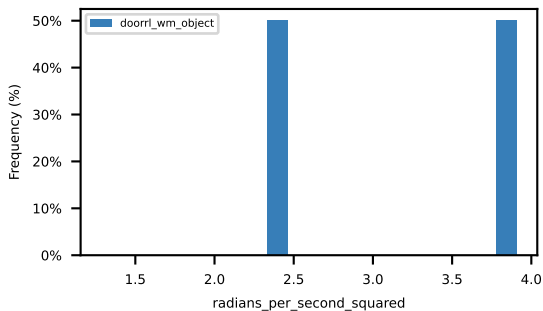
avg_ego_yaw_acceleration
