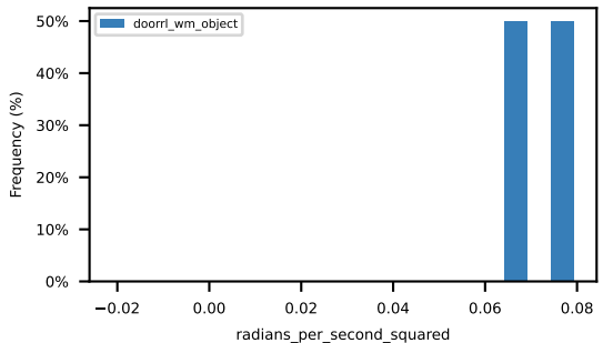
abs_ego_yaw_acceleration_within_bounds
