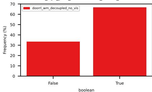
abs_ego_yaw_acceleration_within_bounds
