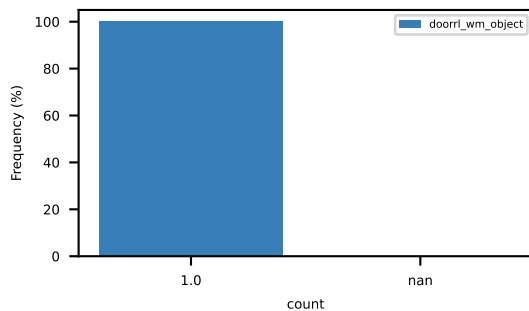
min_violation_of_speed_limit_compliance
