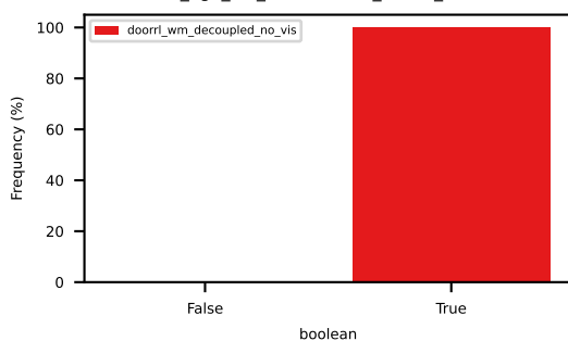
abs_ego_lon_acceleration_within_bounds
