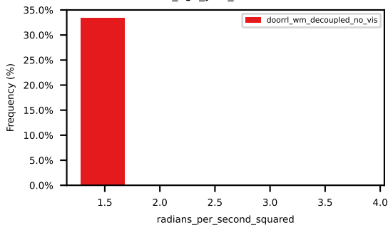
avg_ego_yaw_acceleration
