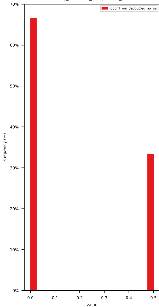
driving_direction_compliance_score
