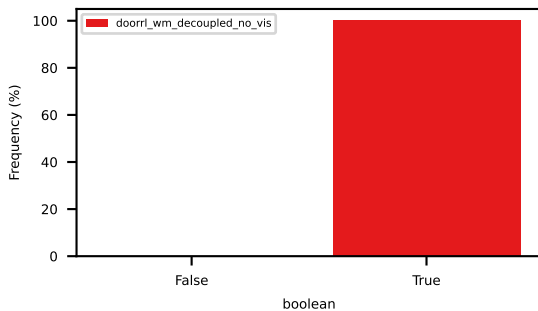
number_of_at_fault_collisions_with_VRUs
