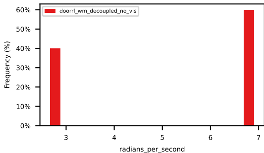
avg_ego_yaw_rate
