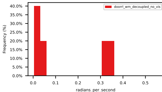
p90_ego_yaw_rate
