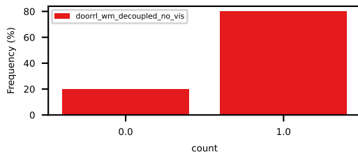
number_of_at_fault_collisions_with_vehicles
