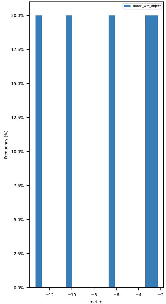
min_progress_along_driving_direction_in_1_second_interval
