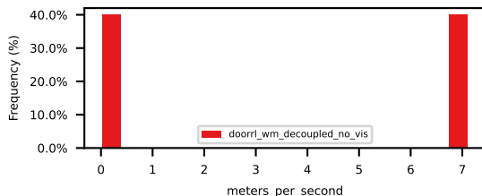
mean_collision_energy_with_vehicles
