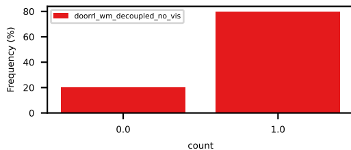
max_collision_energy_with_vehicles
