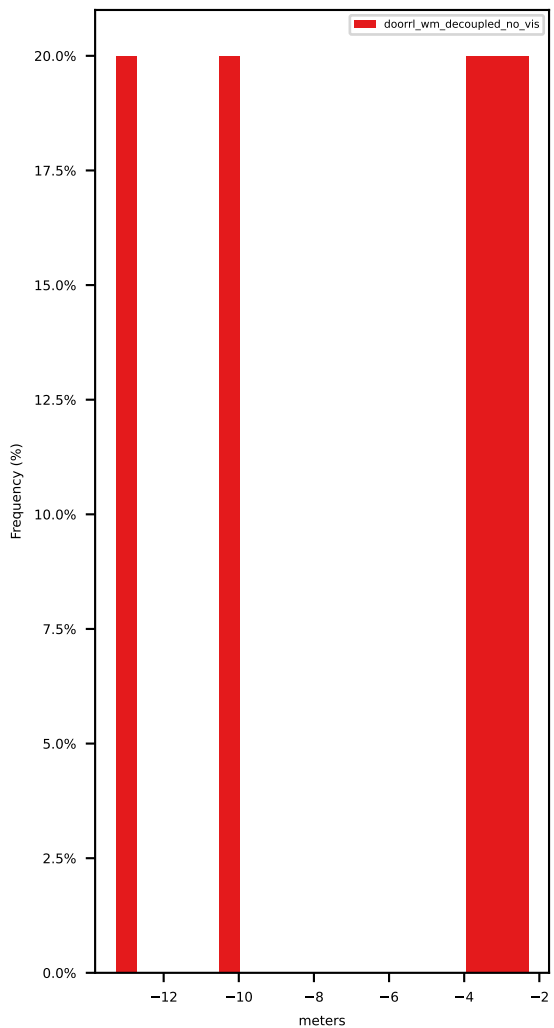
min_progress_along_driving_direction_in_1_second_interval
