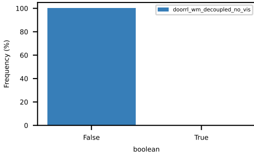
speed_limit_compliance
