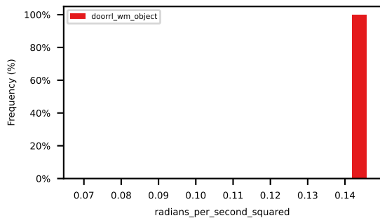
p90_ego_yaw_acceleration
