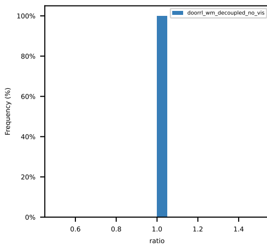
ego_expert_progress_along_route_ratio
