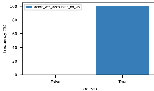
abs_ego_yaw_acceleration_within_bounds
