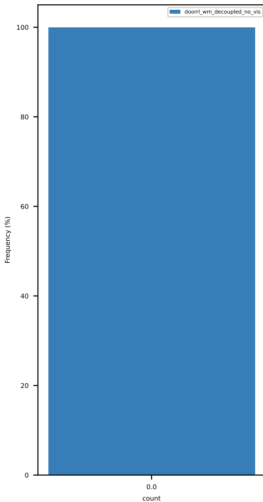
number_of_ego_lane_change
