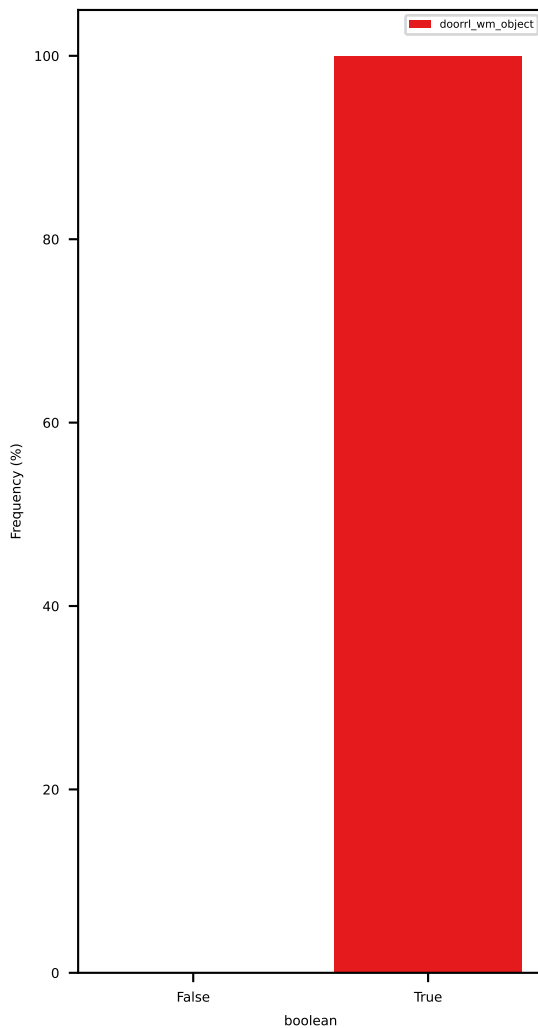
ego_lane_change_fail_rate_below_threshold
