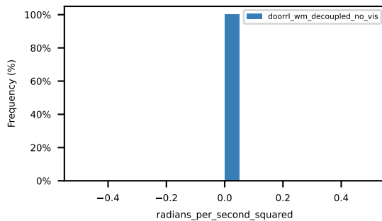
p90_ego_yaw_acceleration
