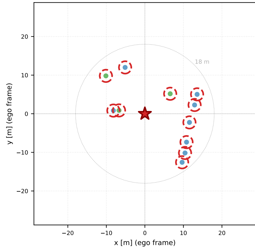
Object+Relation-16 (naive, shared top-k) 0 / 11 near agents selected · pred err = 6.38 m
