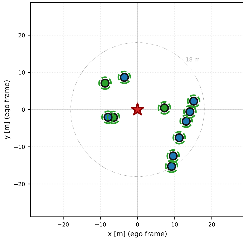
Decoupled typed-budget (Ours, 12 dyn + 4 rel) 11 / 11 near agents selected · pred err = 0.36 m
