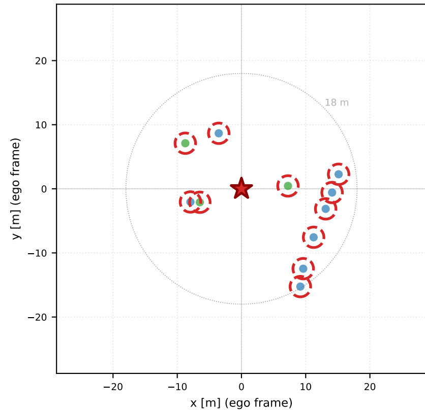
Object+Relation-16 (naive, shared top-k) 0 / 11 near agents selected · pred err = 6.78 m
