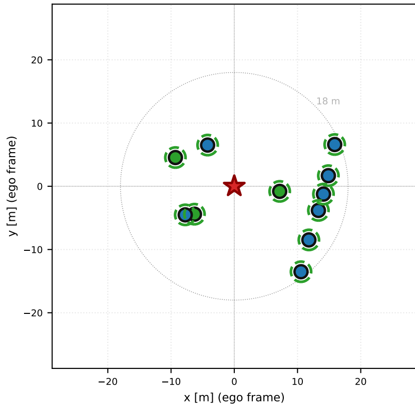
Decoupled typed-budget (Ours, 12 dyn + 4 rel) 11 / 11 near agents selected · pred err = 0.37 m
