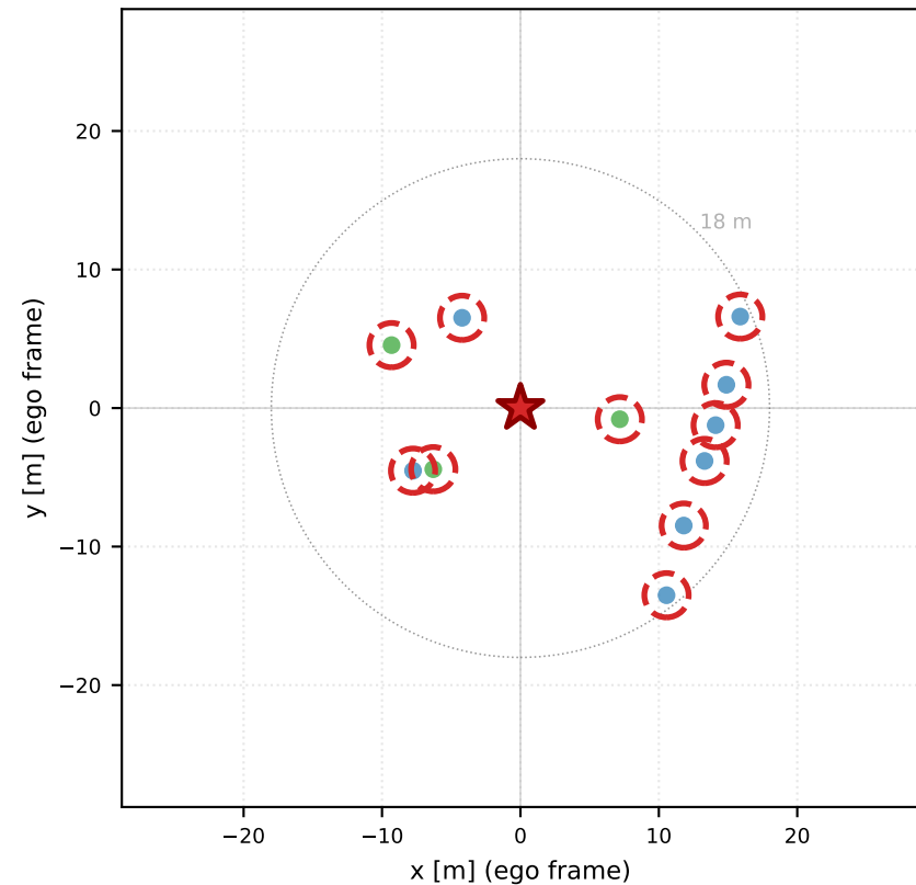
Object+Relation-16 (naive, shared top-k) 0 / 11 near agents selected · pred err = 6.86 m
