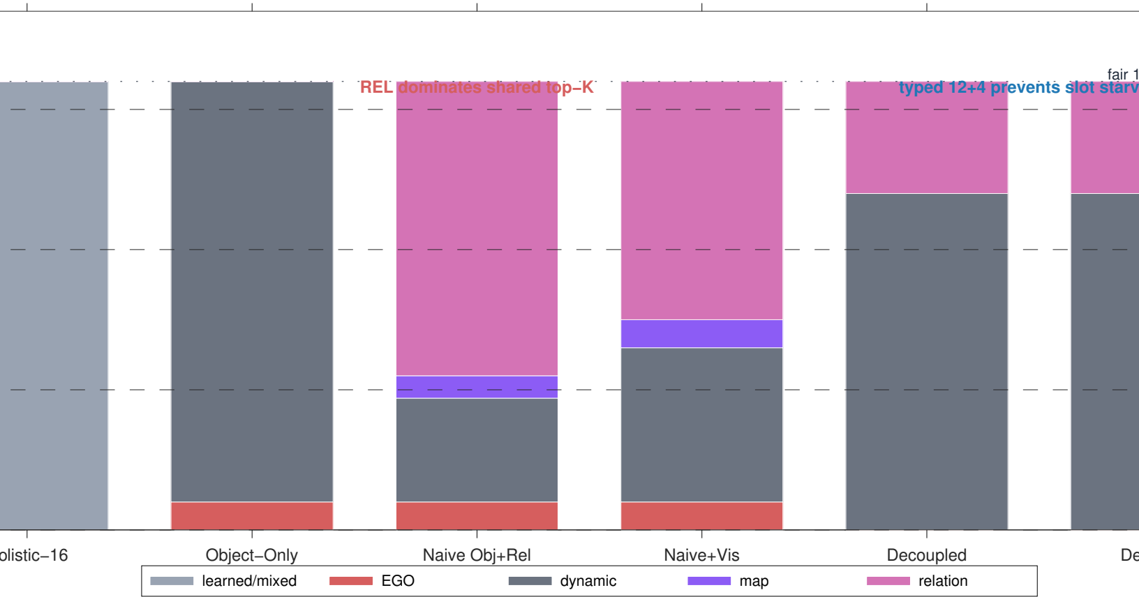
Stage-0 slot-type composition under the fair 16-slot budget
