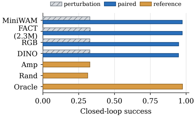
Fig. 6. Closed-loop selection. Paired-geometry training approaches the oracle; perturbation training collapses toward amplitude/random references.
