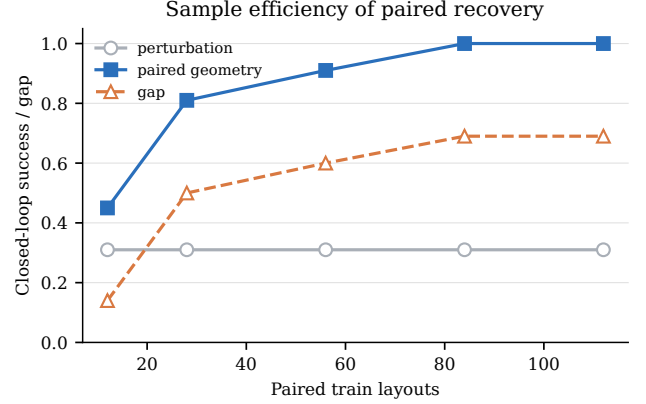
Fig. 7. Paired recovery is data-efficient (gap vs. #paired layouts).
