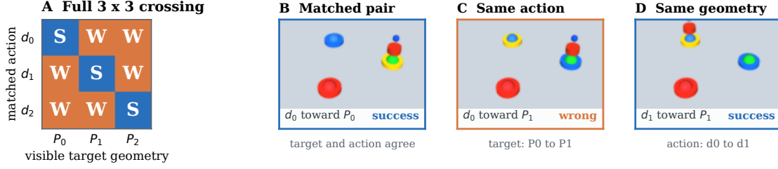
Fig. 3. The complete action×geometry crossing from actual MuJoCo rollouts. Each row holds the candidate action fixed; each column changes only the visible target geometry. The diagonal is the matched-direction success pattern; off-diagonal cells are non-success outcomes.
