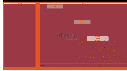
Fig. 3. WordRush minigame
