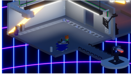
Fig. 2. Game scene
