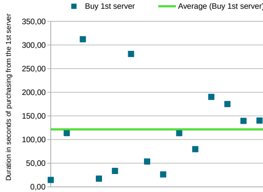
Fig. 4. Time required for players to purchase the first server (high dispersion relative to the mean).
