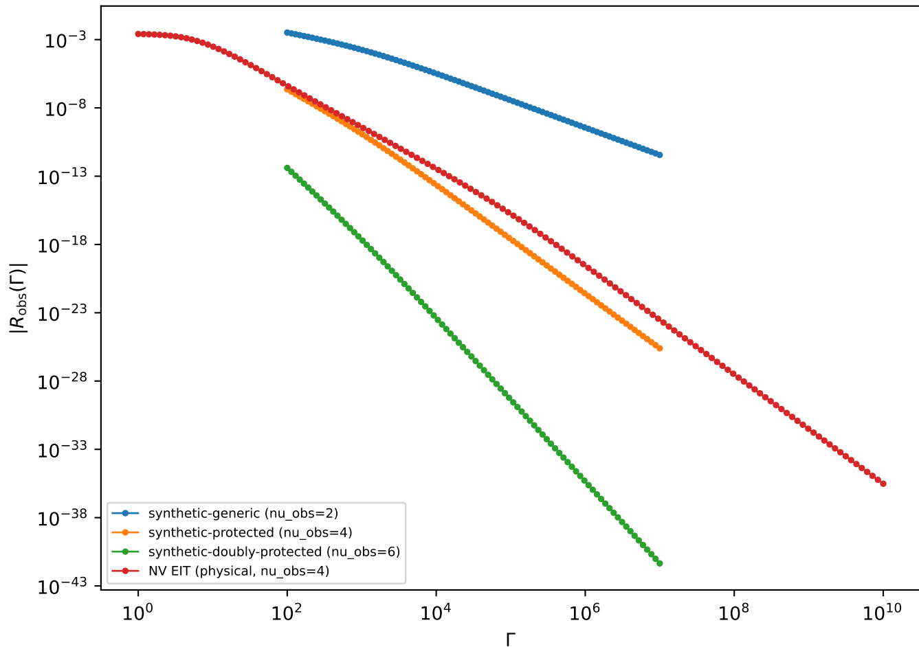
Gate A: observable-order inheritance ( \nu_{\text{obs}} = n_{12} + n_{21} - \nu_{\text{den}} )
