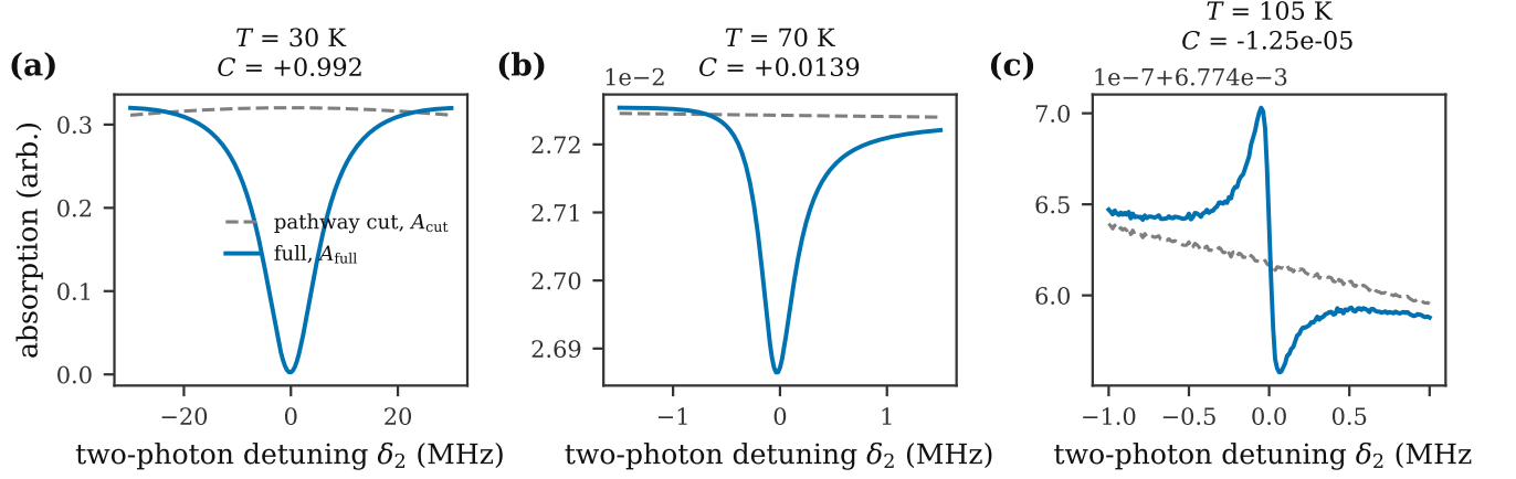
FIG. 2. Full-Liouvillian absorption spectra at the candidate field B_{\perp} = 0.232 T, with the ground-coherence pathway intact ( A_{\text{full}} , solid) and cut ( A_{\text{cut}} , dashed). (a) At 30 K the pathway removes essentially all of the sector absorption. (b) At 70 K a per-cent-level transparency survives. (c) At 105 K the two curves have crossed: the pathway now adds absorption, and the contrast has changed sign.
