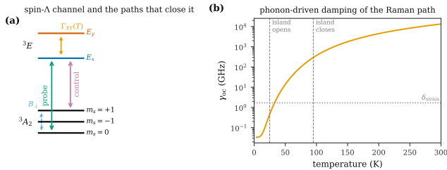
FIG. 1. (a) The \text{NV}^- spin- \Lambda channel. Probe and control address two ground spin sublevels through the {}^3E orbital doublet. Because the optical dipole is orbital, the two legs reach orthogonal spin states and the leading Raman vertex is closed at B_\perp = 0 ; a transverse field mixes the ground sublevels and opens it. Phonon-induced hopping \Gamma_{XY}(T) between the excited branches damps the pathway. (b) Optical-coherence damping \gamma_{oc}(T) over the range studied, with the transverse strain splitting marked for scale. The island boundaries found in Sec. III are indicated.
