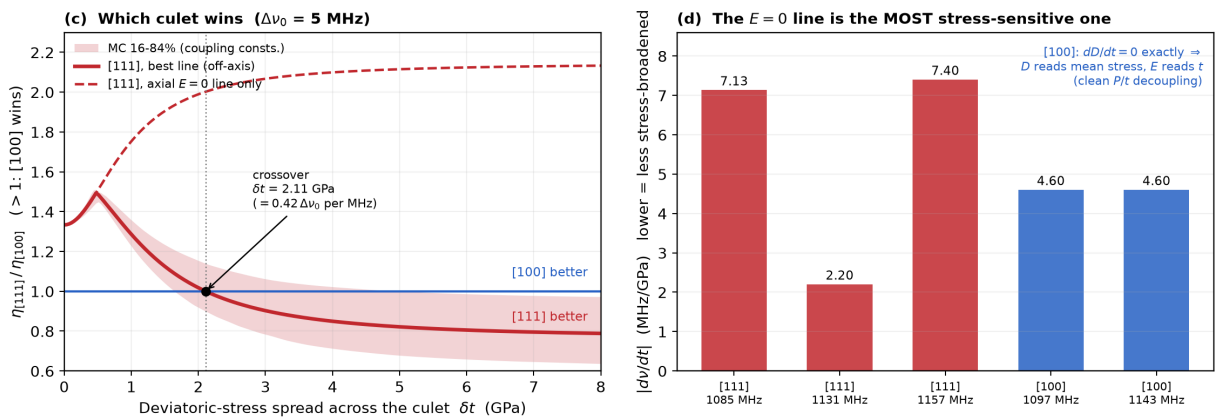
Fig 1: Left: \eta_{[111]}/\eta_{[100]} vs. the deviatoric-stress spread \delta t , for the best [111] line and for the axial E = 0 line alone, with a Monte-Carlo band over the Barson spin-stress constants. Right: |d\nu/dt| of every line; the E = 0 line is the steepest one.
