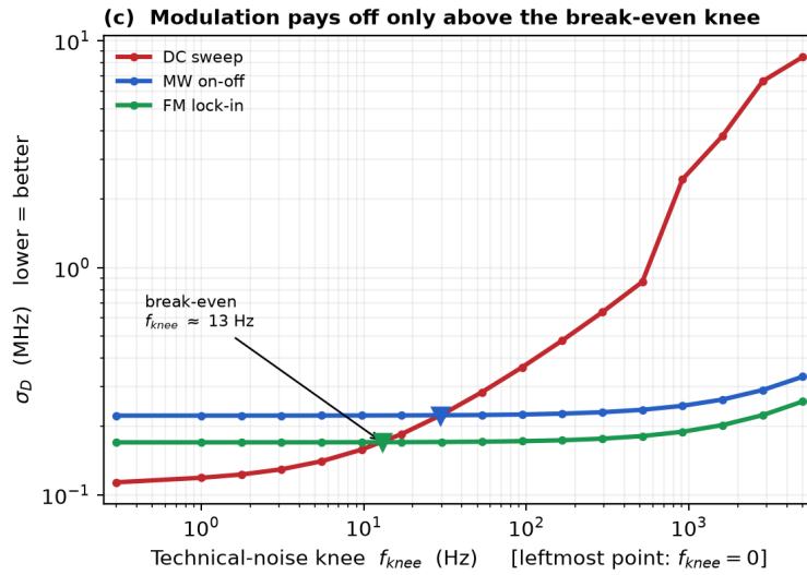
Fig 1: Monte-Carlo \sigma_D (200 realisations, identical total measurement time and identical noise realisation per trial) for a DC sweep, MW on-off chopping and FM lock-in, as a function of the technical-noise knee. Triangles mark the break-even knees.
