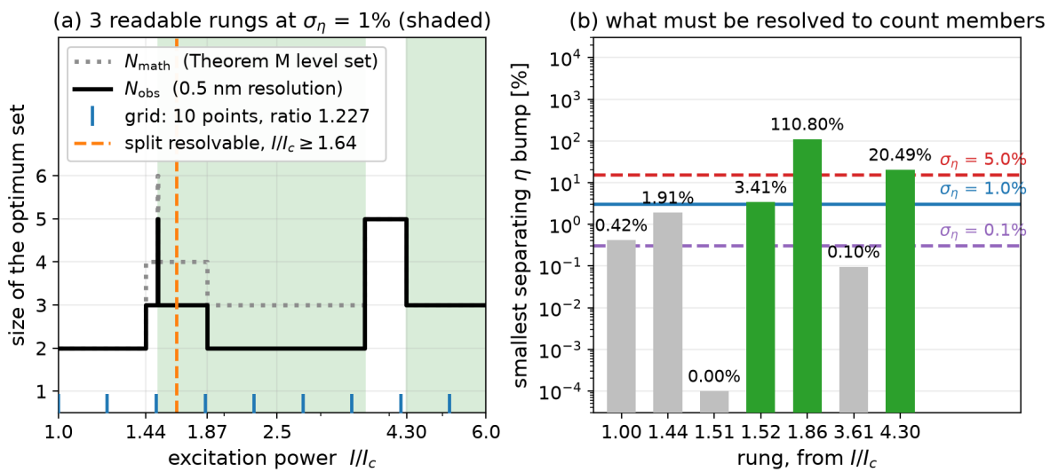
Fig 1: (a) The computed ladder ( N_{\text{math}} ) against the observable one ( N_{\text{obs}} , members within 0.5 nm merged); shaded rungs are readable at \sigma_\eta = 1\% . (b) The smallest \eta bump on each rung against the 3\sigma floor.
