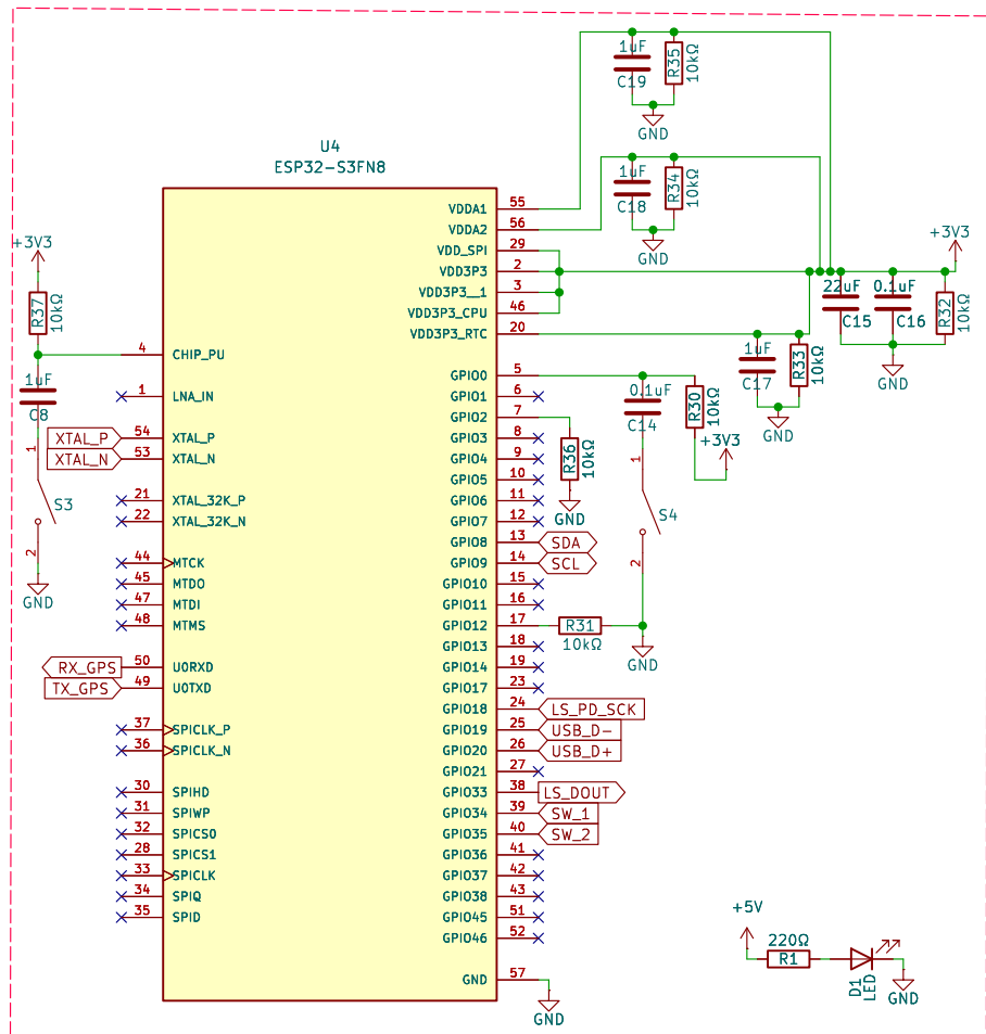
Micro-Controlling Unit
