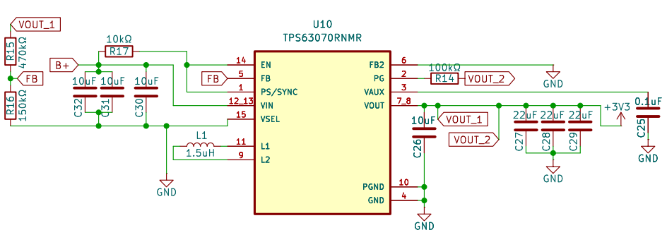
Buck/Boost Converter
