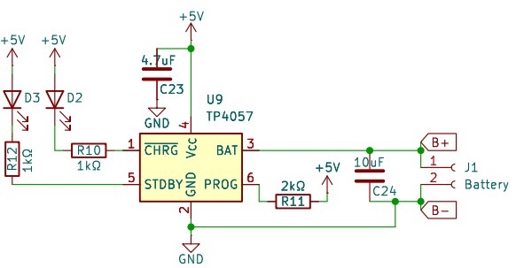
Battery Charging Unit
