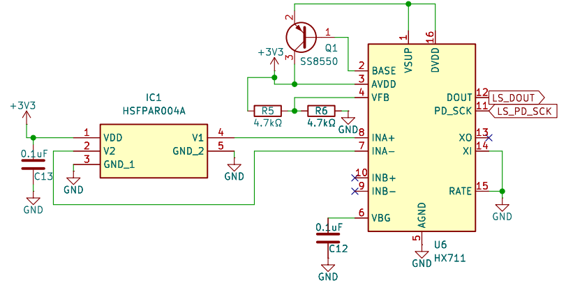
Load Sensing Unit
