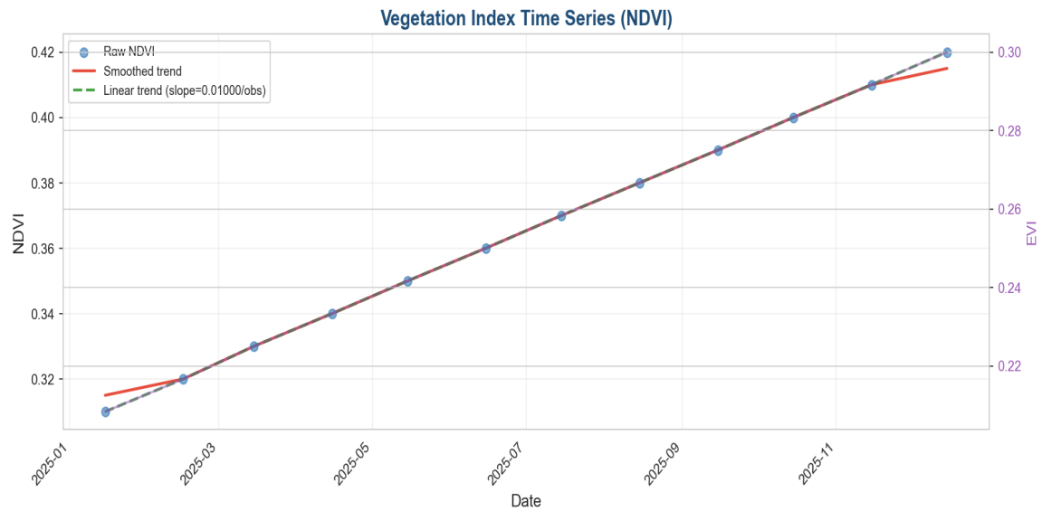
Figure 3: NDVI Time Series with Trend
