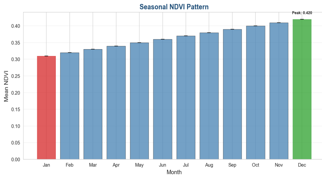
Figure 4: Monthly Seasonal NDVI Pattern
