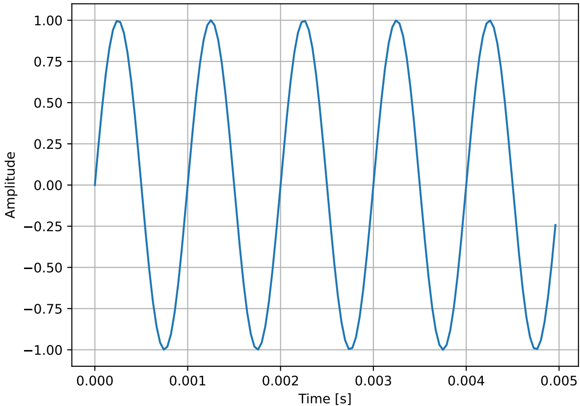
Simple Sine Wave
