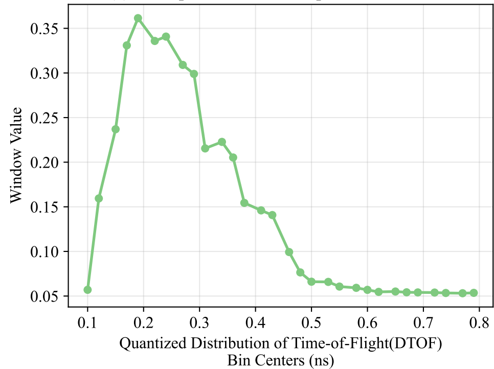
(a) Example of a DIGSS-Optimized Window
