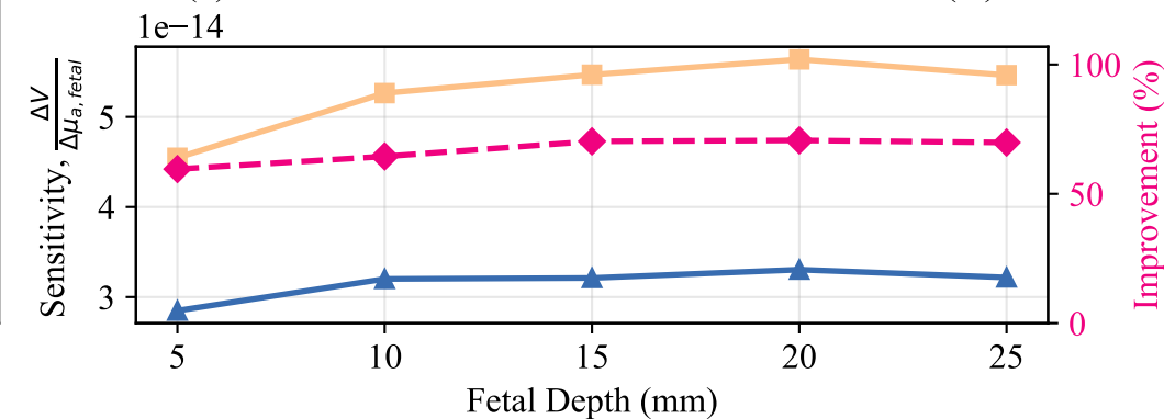
(c) Measurand: Photon Arrival Time Variance ( V )
