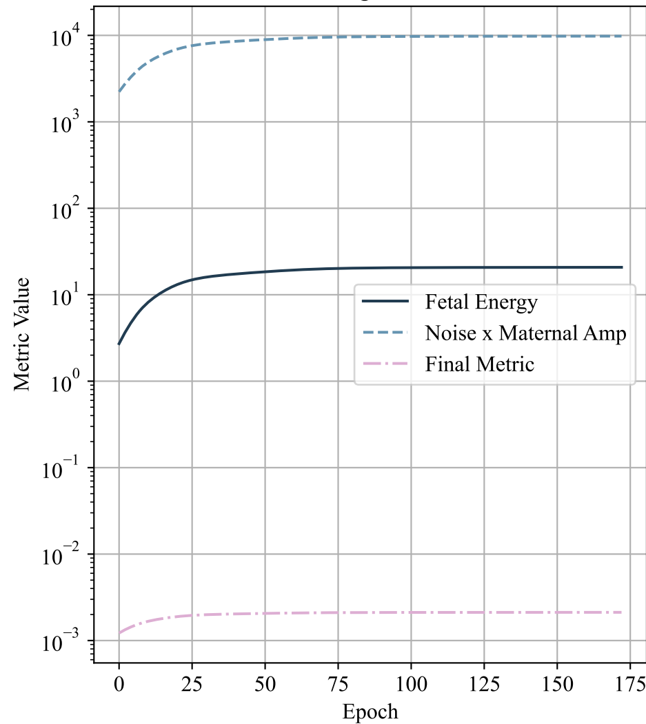
Training Metrics
