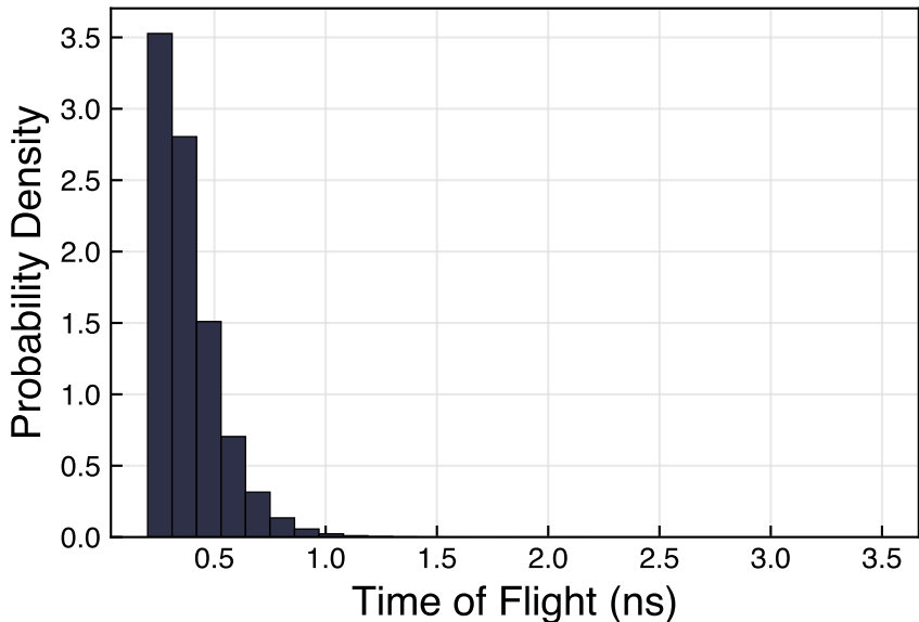
Distribution Time-of-Flight (DTOF)
