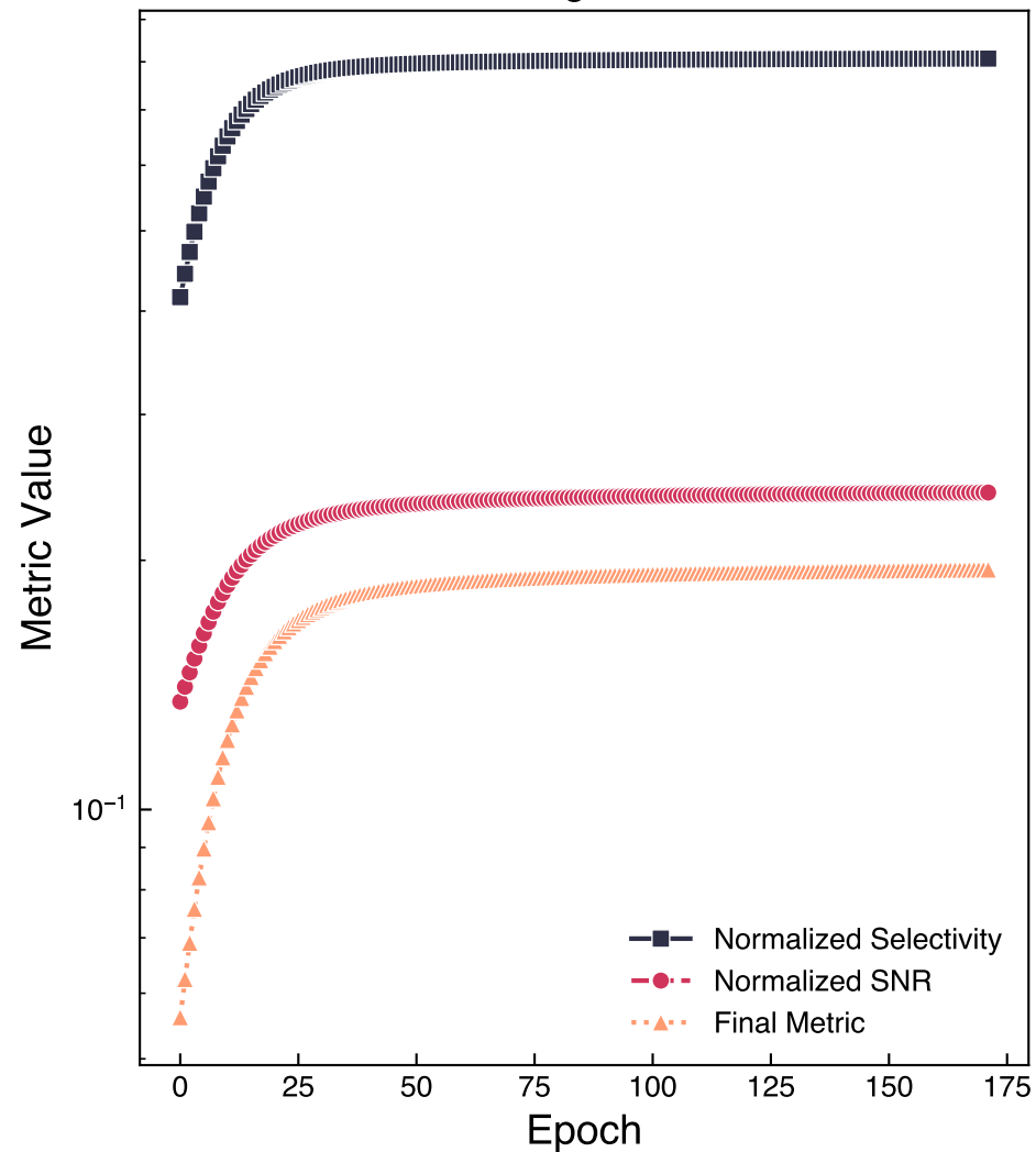
Training Metrics
