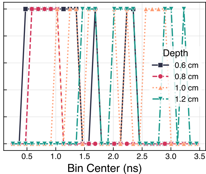
DIGSS(Unit Max)
