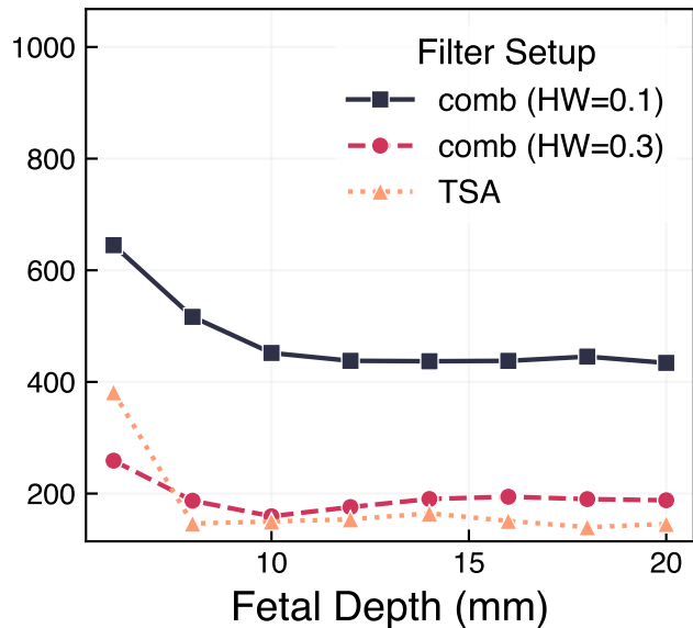
Reward Metric
