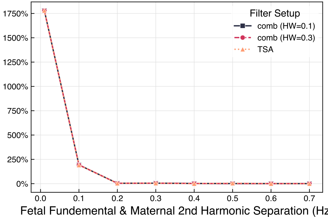
FoM & Reward Metric Mismatch
