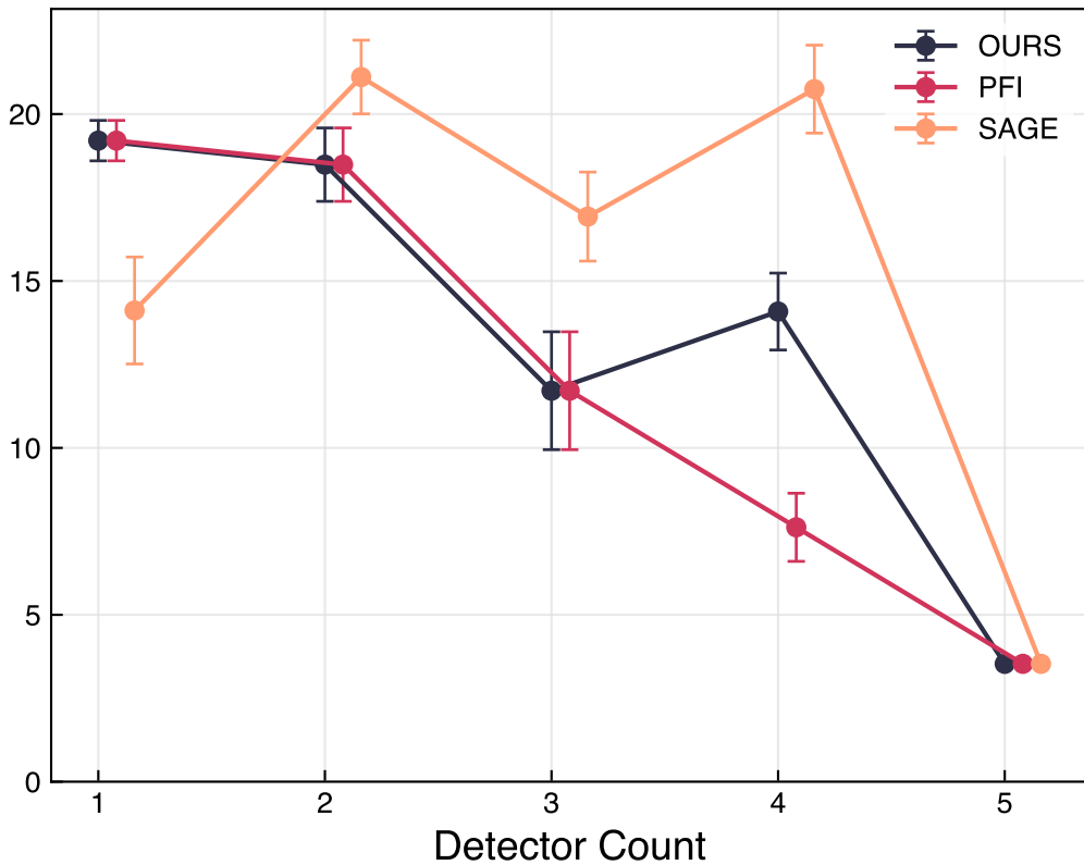
Test Error (MAE % Saturation)
