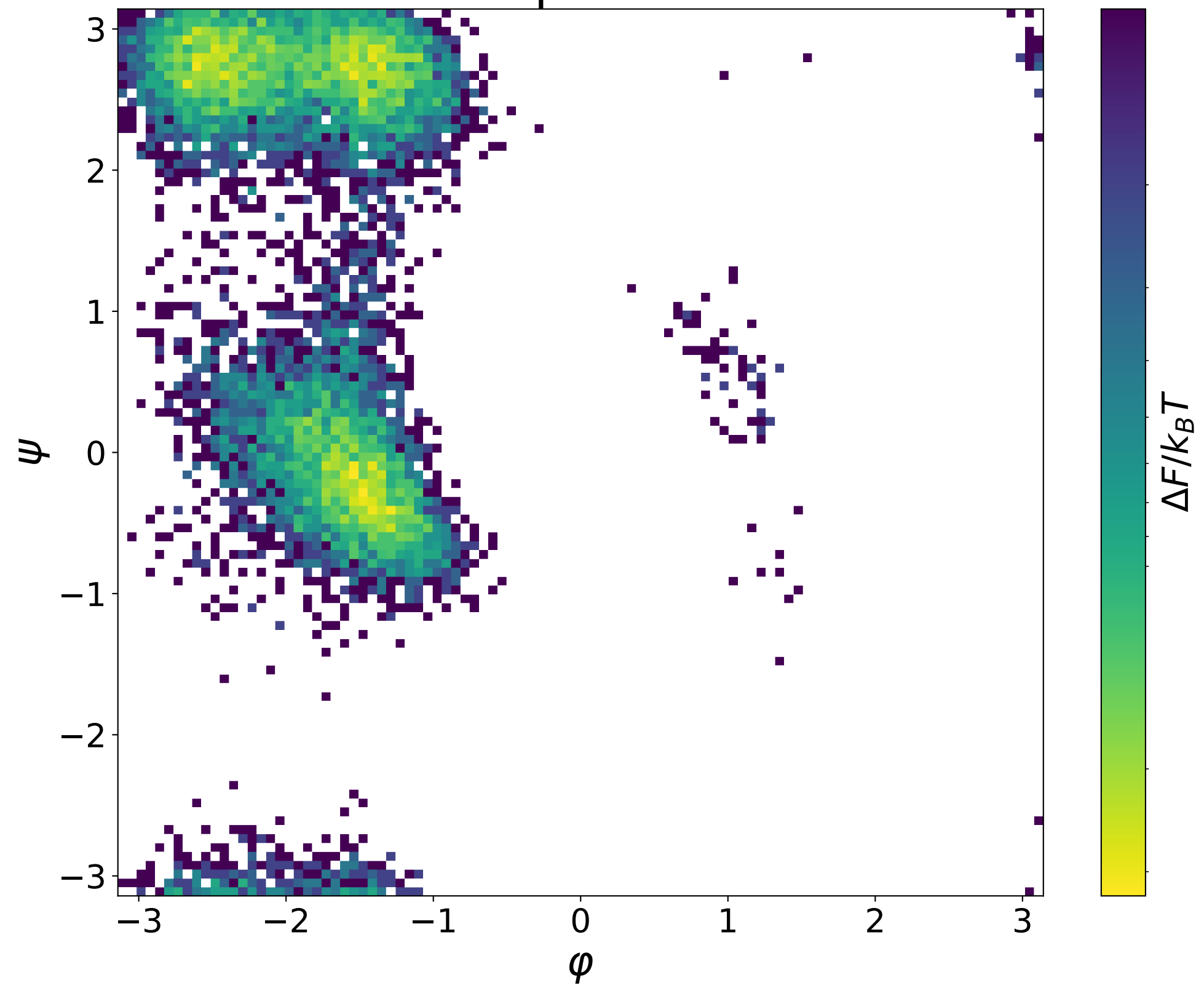
MD relaxed samples Ramachandran
