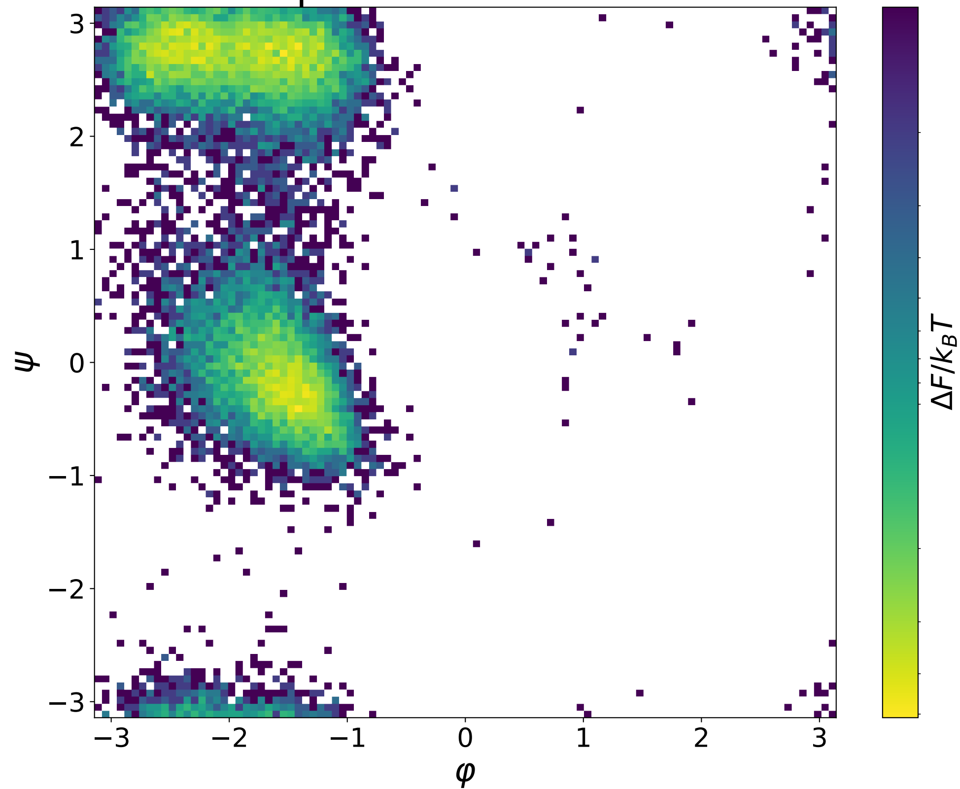
endpoint Ramachandran
