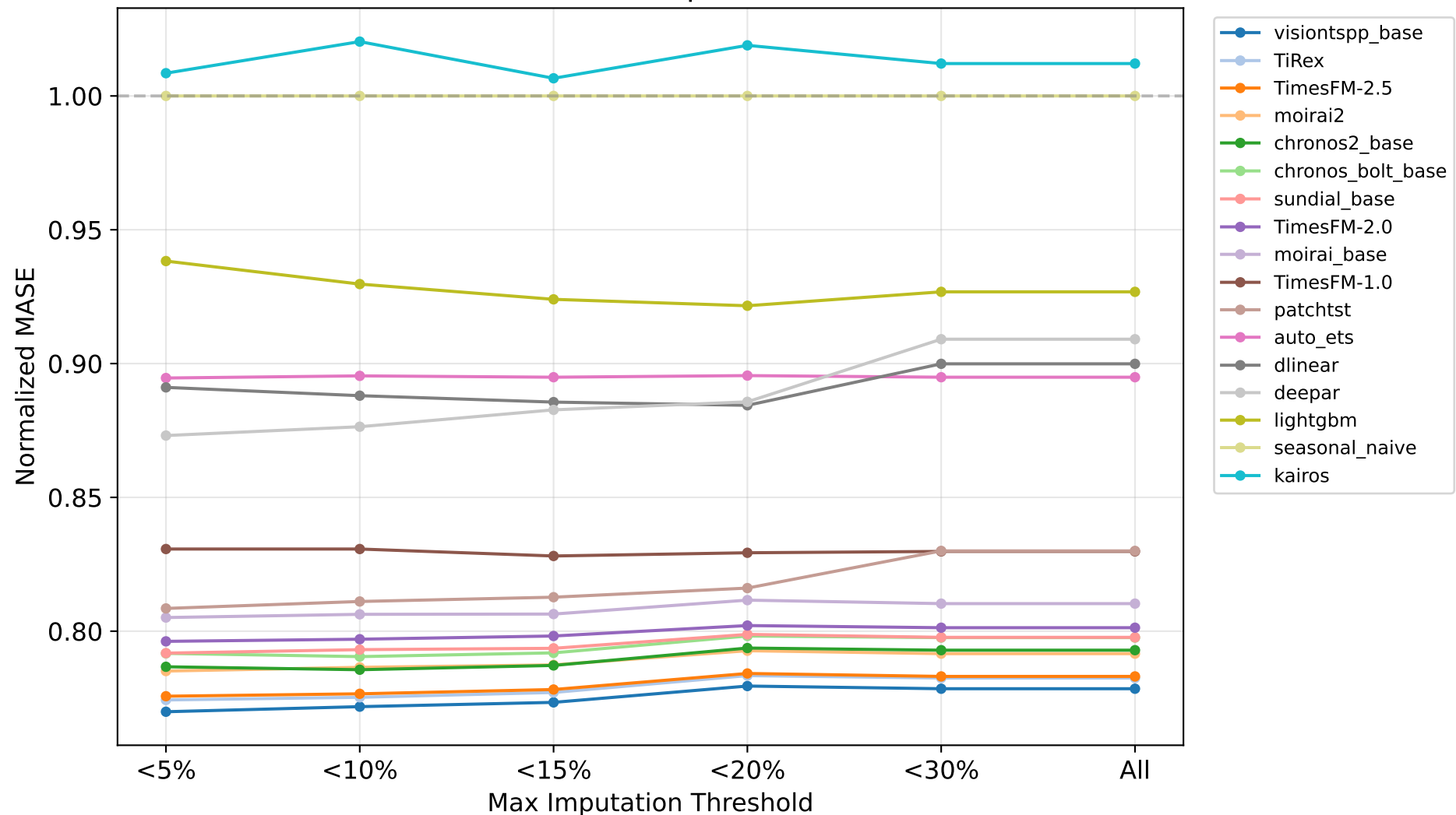
Normalized MASE vs Imputation Threshold
