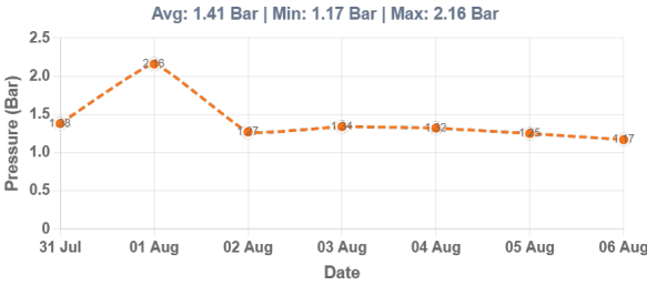
ESR Ganganagar - 1.34 LL - Pressure Levels (7 Days)
