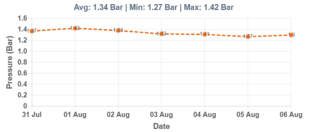
ESR Nageshwarnagar- 3.73 LL - Pressure Levels (7 Days)
