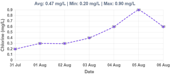
ESR Ganganagar - 1.34 LL - Chlorine Levels (7 Days)
