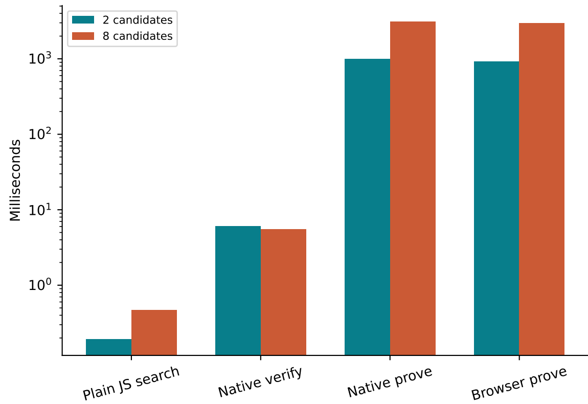
Groth16 calibration: reduced contact model
