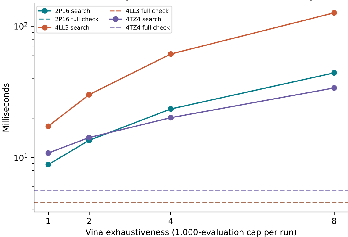
Real docking: warmed native search and checking
