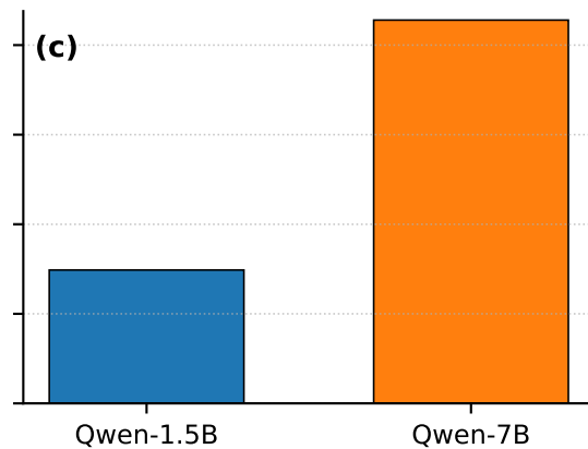
MMLU-physics
