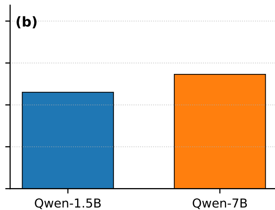
MMLU-math
