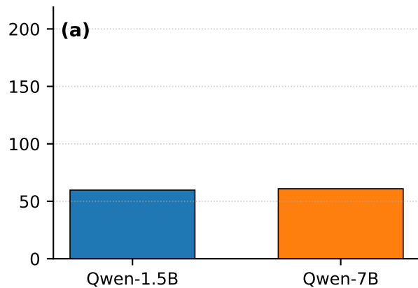
MATH-500
