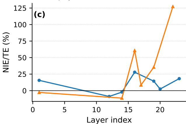
MMLU-physics
