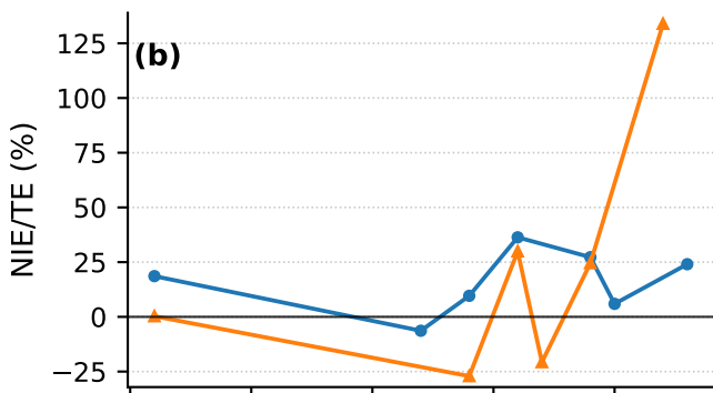
MMLU-math
