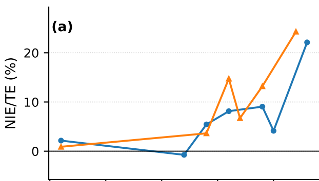
MATH-500
